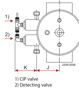
1) CIP valve 2) Detecting valve c. Top view
